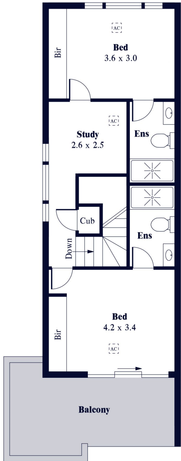
First Floor
